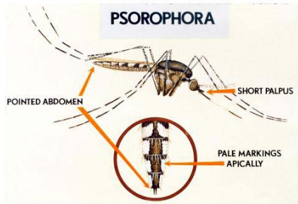
5A. Psorophora spp.
